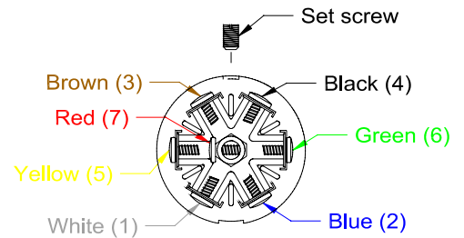
Plug, 7 Blade, Wiring Diagram.
